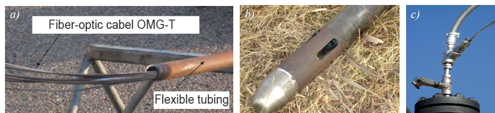
Fig. 8. Flexible tubing (a, b) with a diameter of 1.25" for the installation of T-P sensors in the well; (c) Cable entry at the wellhead ( www.weatherford.com )
